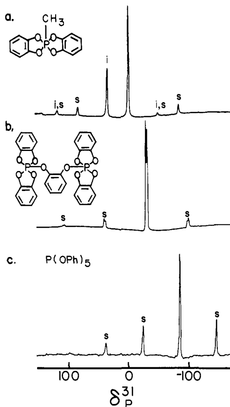
Figure 2. Representative 31 P NMR spectra of solid samples of penta-coordinated phosphorus compounds. Spinning side bands are indicated by "S". Impurities are indicated by "I". Parameters: (a) 1.5 ms contact time, 8 s repetition rate, 250 scans, (b) 9.5 ms contact time, 8 s repetition rate, 2610 scans, (c) 9 ms contact time, 12 s repetition rate, 372 scans.
